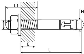
Standard: Wedge Anchor
