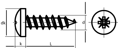
Standard: Din7505-B (Pozi Drive)
