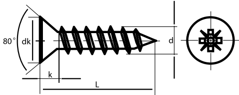
Standard: Din7505-A (Pozi Drive)
